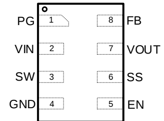
Top View: QFN-8L 1.5mm x 2mm, Plastic
