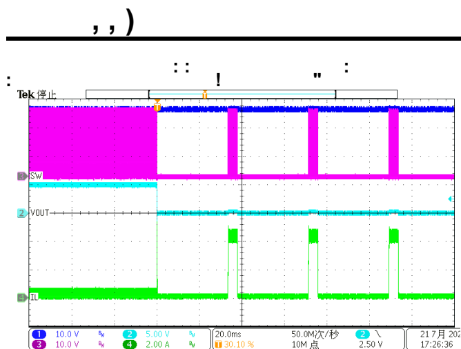
Figure 18. Over Current Protection(OA to hard short)
