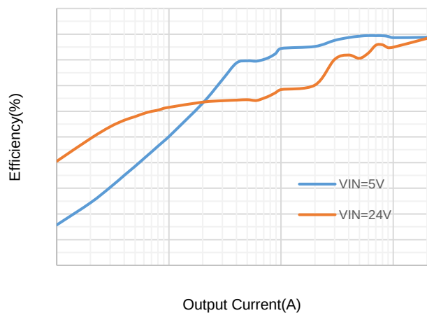
Figure 6. Efficiency vs Load Current, Sepic, VOUT=24V
