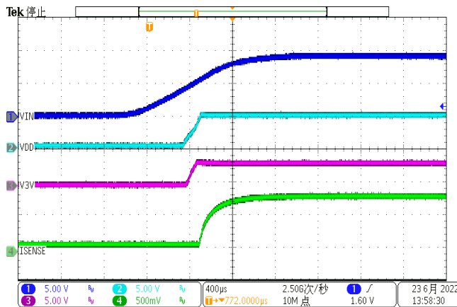
Figure 12. Power Up
