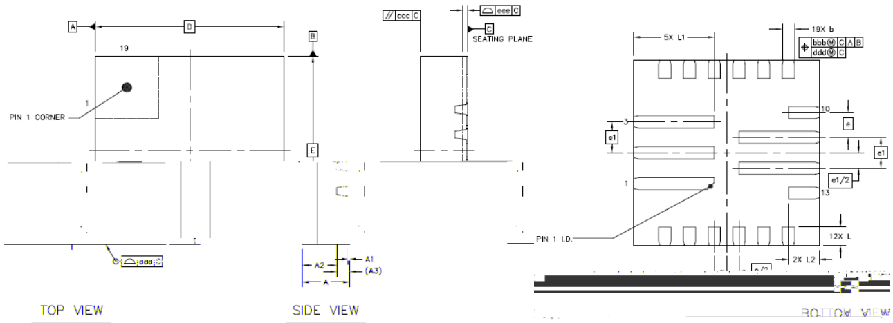
FCQFN-19L (3x3) Package Outline Dimensions
