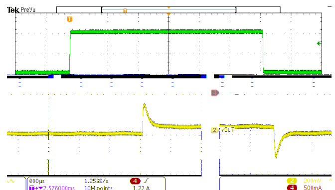
Figure 18. Load Transient VOUT=5V, IOUT=0.5A to 1.5A, SR=250mA/us
