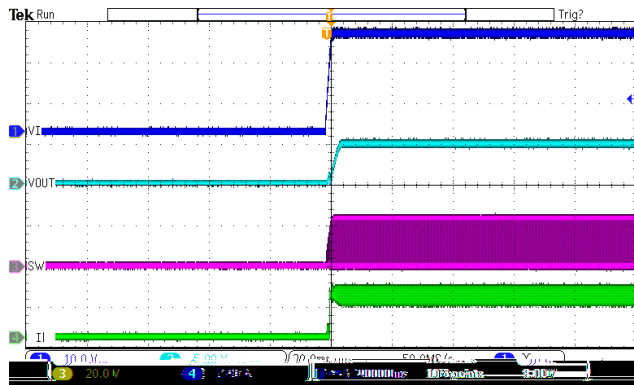
Figure 15. Power Up VIN=24V, VOUT=5V, IOUT=2A
