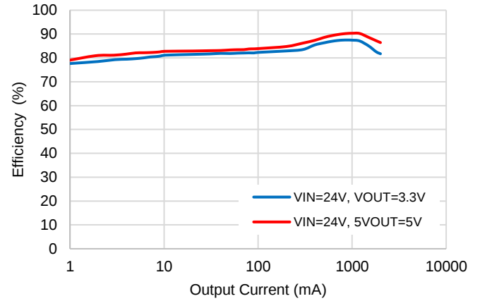
Figure 2. SCT9320 Efficiency, Vin=24V
