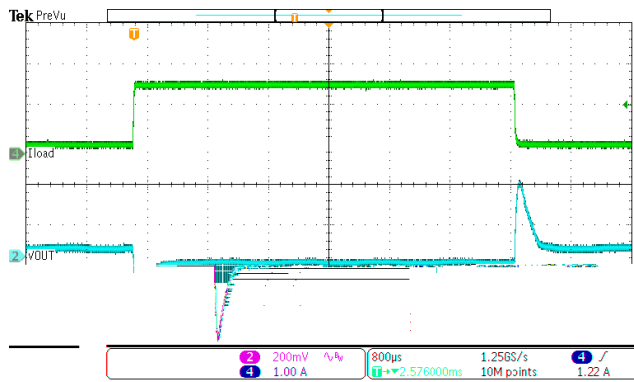
Figure 17. Load Transient VOUT=5V, IOUT=0.2A to 1.8A, SR=250mA/us
