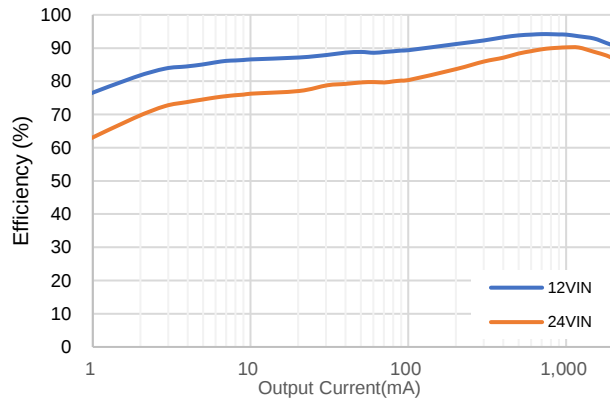
Figure 1. Efficiency, Vout=5V
