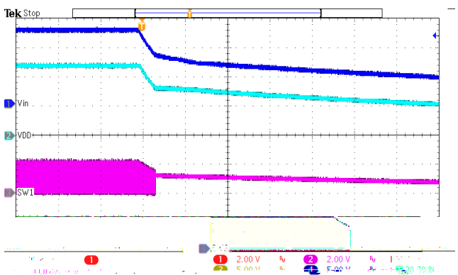
Figure 9. Power Down
