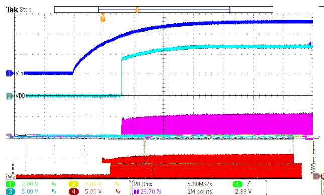
Figure 8. Power Up
