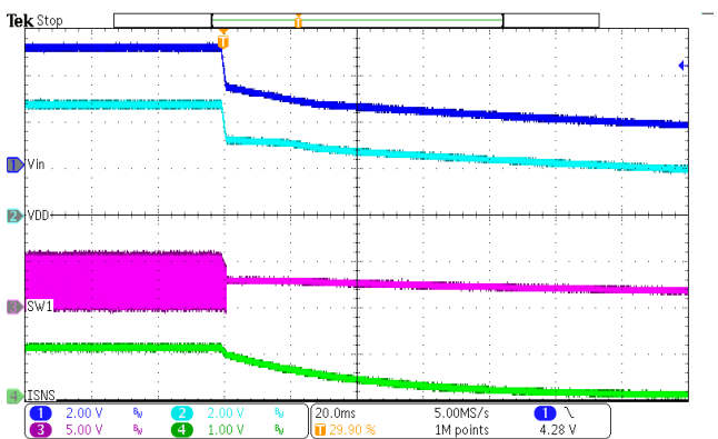
Figure 11. Power Down
