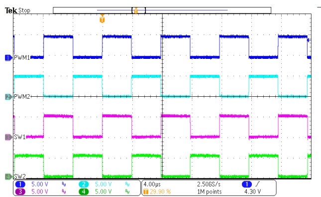
Figure 12. Full bridge @ Vin=5V, RX=5W
