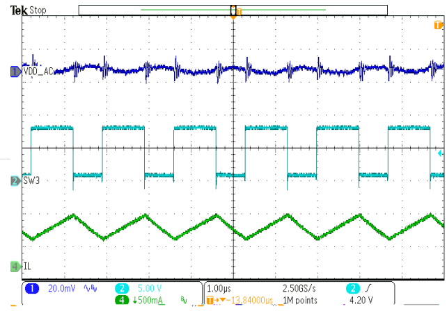
Figure 15. VDD Ripple and SW3 @VIN=9V, IOU=600mA
