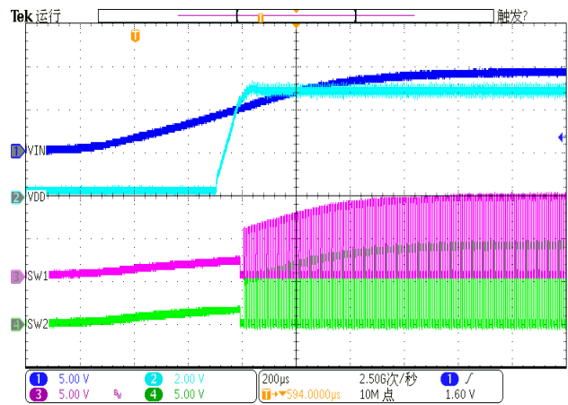
Figure 13. Power Up
