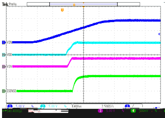
Figure 12. Power Up
