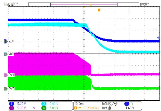
Figure 15. Power Down
