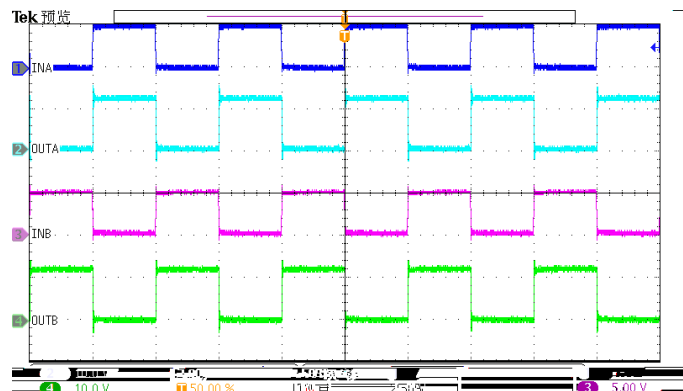
Application Waveform
