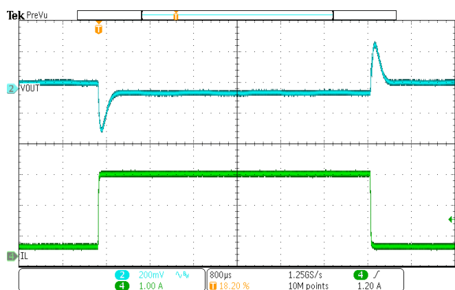
Figure 20. Load Transient VOUT=5V, IOUT=0.3A to 2.7A, SR=250mA/us
