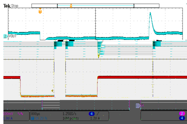
Figure 21. Load Transient VOUT=5V, IOUT=0.75A to 2.25 A, SR=250mA/us
