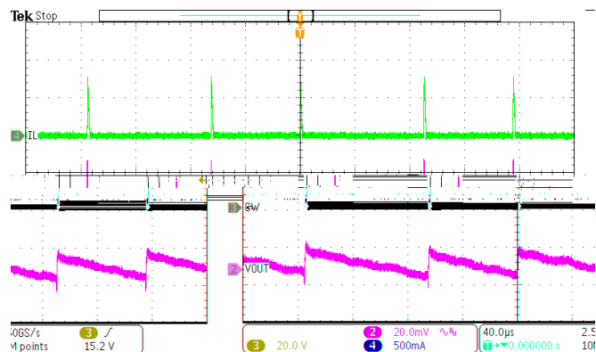
Figure 17. SW node Waveform and Output Ripple VIN=24V, IOUT=10mA
