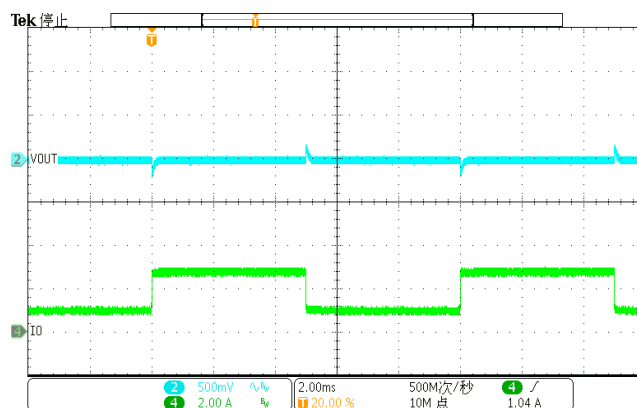
Figure 19. Load Transient (0.87A-2.63A, 1.6A/us)
