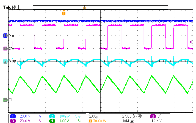
Figure 36. steady-state ( I_{load}=2A )
